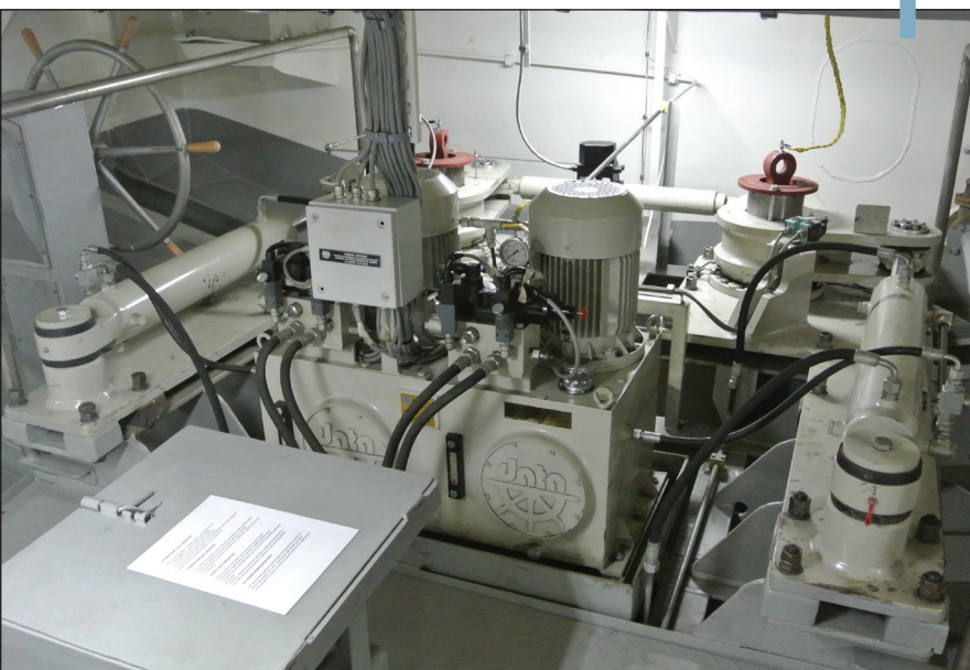
DDM 2x4000 custom design steering gear on a ferryboat
