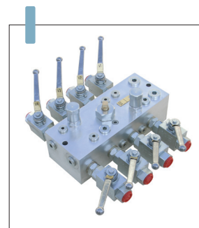
DRB-8, 4 in-4 out, Ports BSP 3/8", 1/2" or 3/4"
