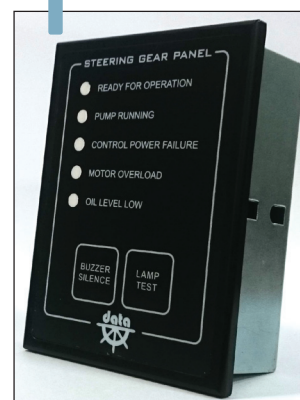
SAP-S Steering gear pump alarm panel
