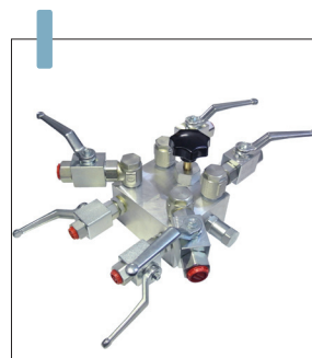
DRB-6, 2 in-4 out, Ports BSP 3/8, 1/2" or 3/4"
