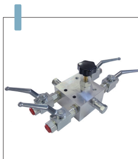
DRB-4, 2 in-2 out, Ports BSP 3/8" or 1/2"
